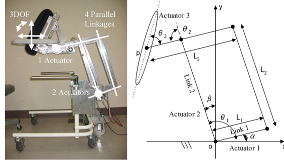
(a) Prototype system (b) Parallel Linkage Mechanism
