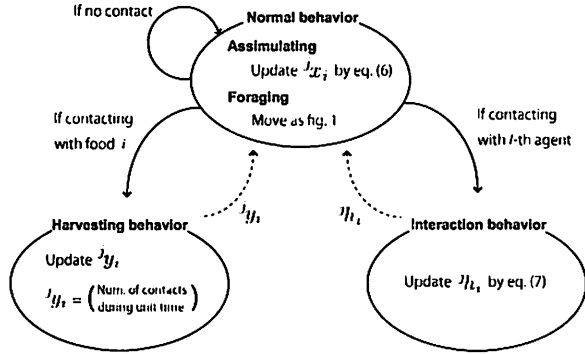
Fig. 3. Transition rules of robot's behavior.
