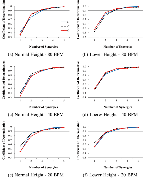
Fig. 3. Change of Coefficient of Determination.
