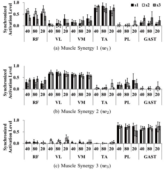
Fig. 4. Extracted Synergies at Normal Height.
