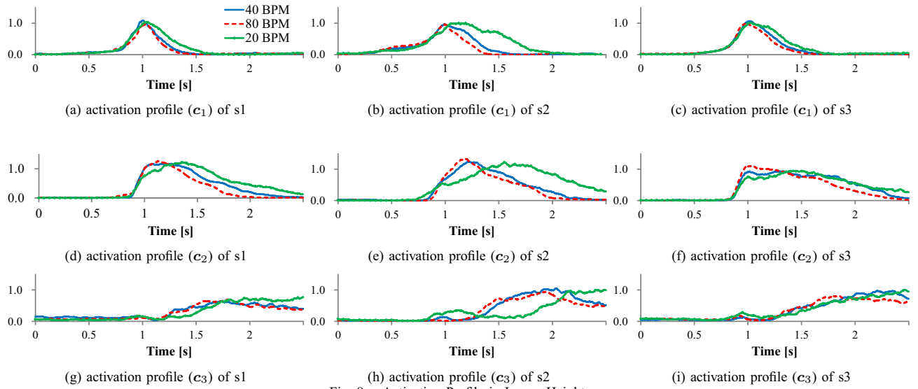
Fig. 8. Activation Profile in Lower Height.
