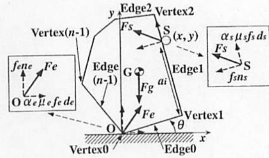
Fig. 16. 2-D model of an object. The formulation is done according to the quasi-static analysis.
