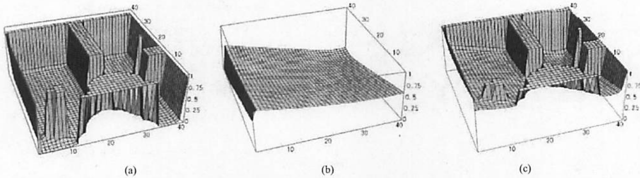
Fig. 12. Potential field. (a) P_{rep} . (b) P_{att} . (c) P_w .
