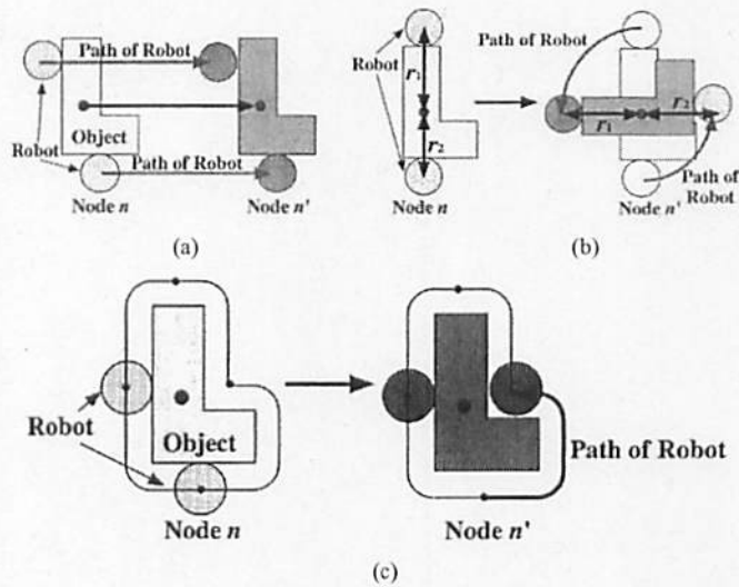
Fig. 10. Constraints and individual robot motions in the primitive operations. (a) Position change operation ( C_{pos} ). (b) Orientation change operation ( C_{ori} ). (c) Arrangement change operation ( C_{arr} ).
