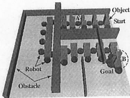
Fig. 23. Simulation results. Result of global path planning.
