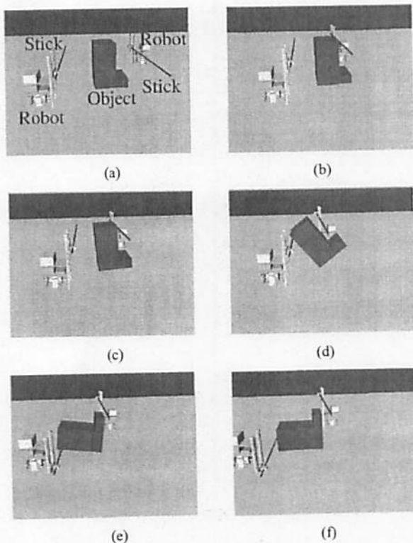
Fig. 24. Simulation results. Result of local manipulation planning at point A in Fig. 23.
