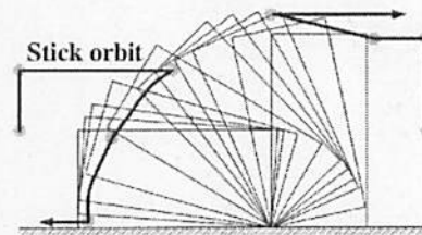
Fig. 22. Orbit of sticks in the case (planning result with motion errors) of Fig. 21(b).
