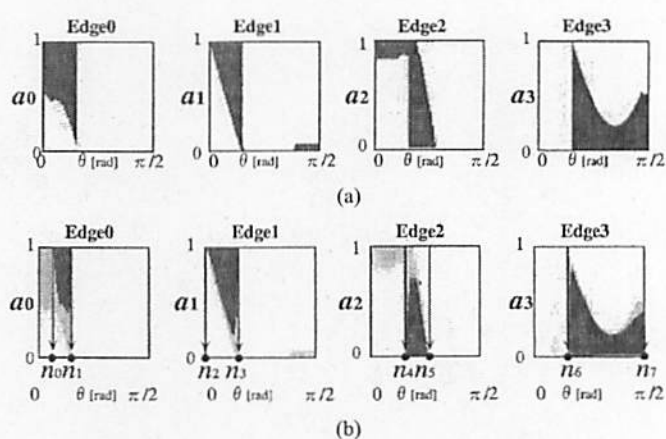
Fig. 18. Stable domain graph of each edge. (a) Stable domain graph without errors. (b) Stable domain graph with errors.
