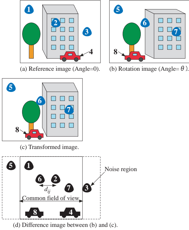
Fig. 3. Projective transformation and difference between two images.
