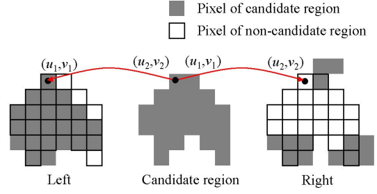
Fig. 4. Judgment by pixel correspondence.
