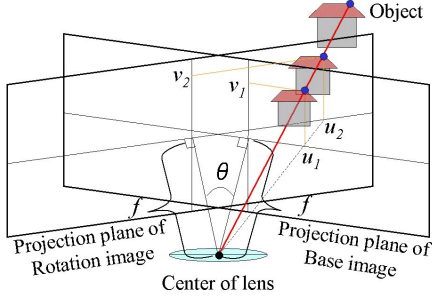
Fig. 2. Projective transformation.
