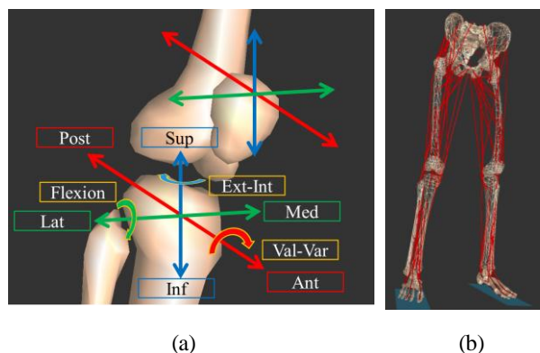
Figure 1 (a) Model coordination such as anterior (Ant), posterior (Post), medial (Med), lateral (Lat), superior (Sup), Inferior (Inf), flexion, external (Ext), internal (Int), valgus (Val), and varus (Var). (b) Overall model.
