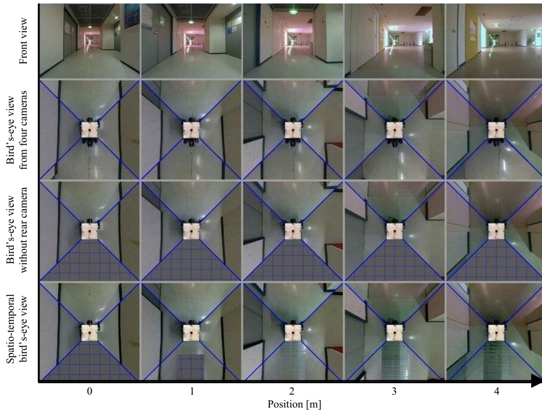
Fig. 10: Result of images. Bird's-eye view images are created from four cameras so that if images are not available, there are blind spots. Spatio-temporal bird's-eye view compensates these blind spots by using past stored images.
