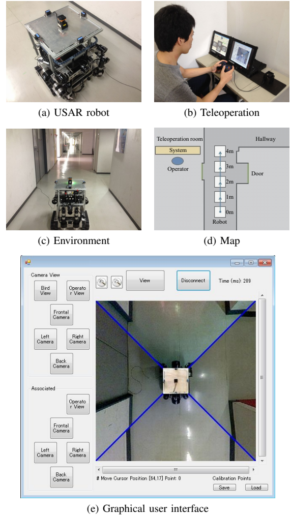
Fig. 9: Teleoperation system and experimental environment.
