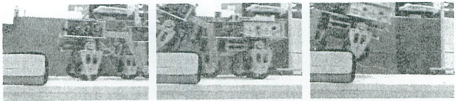
Fig. 9. Passing over the 152[mm] height step
