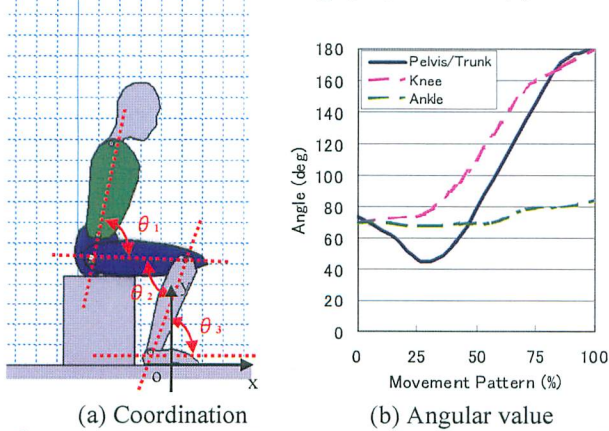
Fig. 5 Standing-up motion with Kamiya scheme \theta_1 shows the angular of the pelvis and the trunk. \theta_2 and \theta_3 shows the angular of the knee and the ankle, respectively
