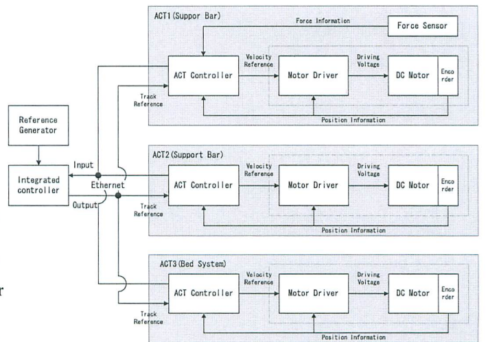
Fig. 3 The structure of our controller
