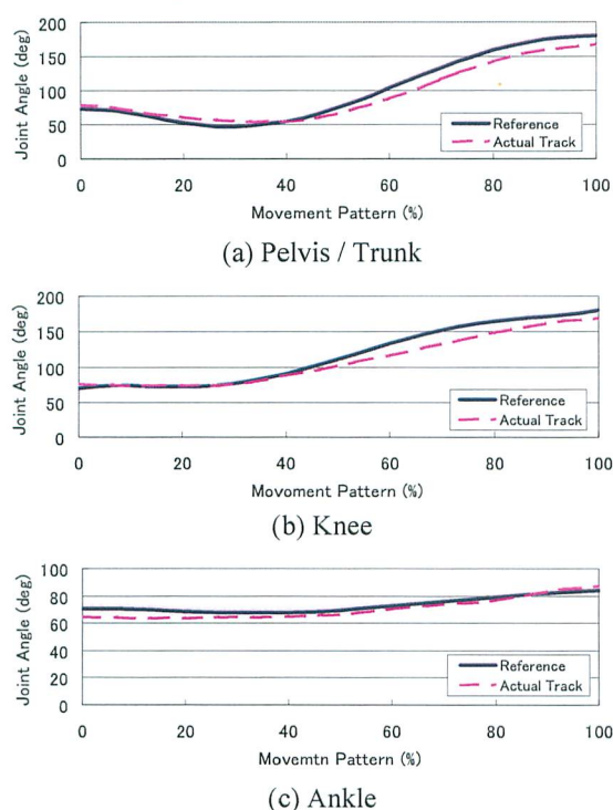
Fig. 13 Angular value of each joint
