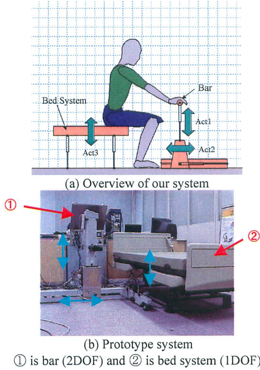
Fig. 1 Our assistant system
