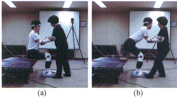
Fig. 4 Standing-up motion with Kamiya scheme
