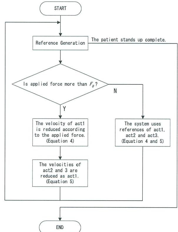
Fig. 9 Flow chart of our proposed control scheme
