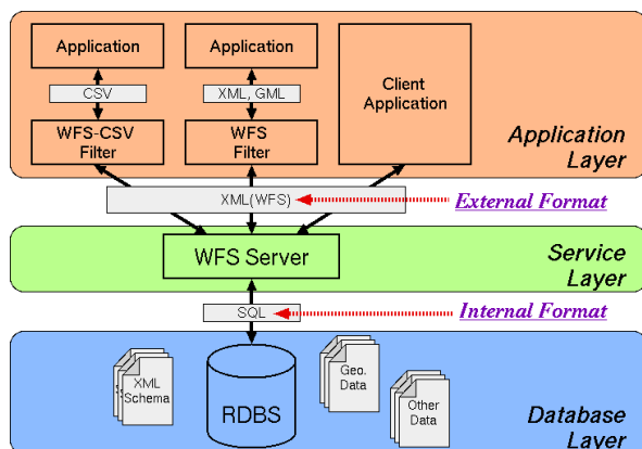
Figure 8 Structure of DaRuMa Database
