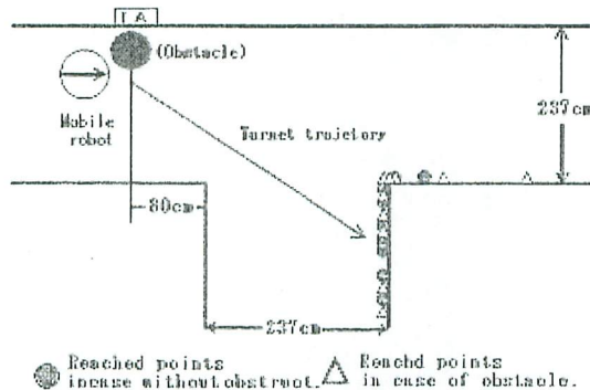
Fig. 2. Experiment of mobile robot operation using IA
