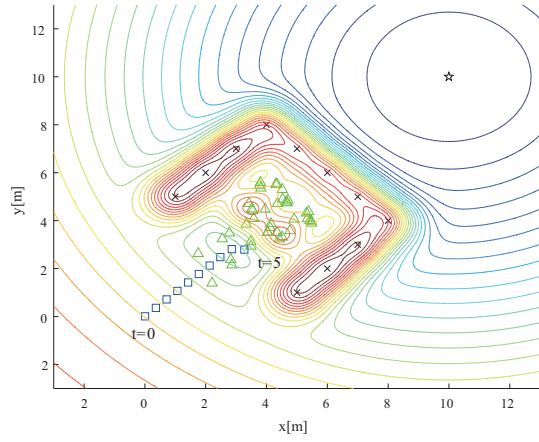
(a) From t = 0 to t = 5
