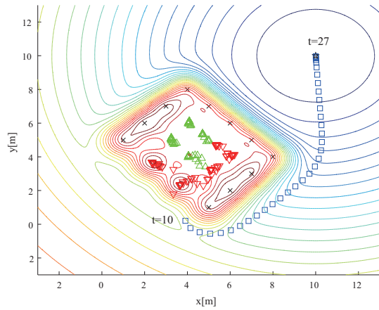
(c) From t = 10 to t = 25
