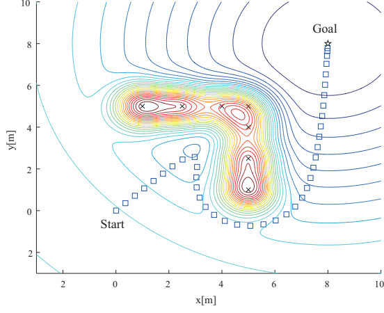
(a) Circumvent motion
