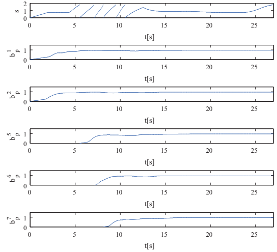
Fig. 5. Transition of internal parameters
