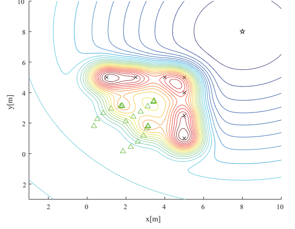
Fig. 2. Contour of potential function compensated by three particles
