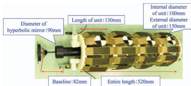
Fig. 1. Earthworm robot equipped with omni-directional rangefinder.
