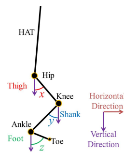
Fig. 1 Elevation angle.
